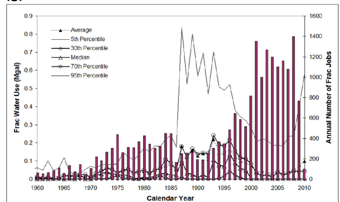
Figure 3. Annual number of HF jobs (columns, right-hand side, vertical axis) superimposed to annual average, median, and other percentiles of individual well frac water use (lines, left-hand-side, vertical axis) for (a) Barnett vertical wells, (b) Barnett horizontal wells, (c) Anadarko Basin, (d) East Texas Basin (mostly Cotton Valley), (e) Permian Basin, (f) Permian Basin (>0.1 Mgal only), and (g) Gulf Coast.
