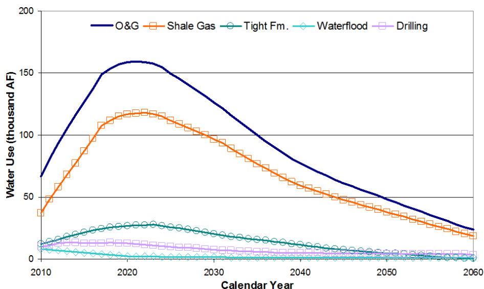
Figure 8. Summary of projected water use in oil and gas segment (2010–2060), including statewide water use for shale and tight-formation plays (whose sum is displayed in Figure 7), waterflood, and drilling.
